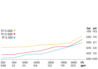
Pressure Loss
