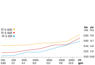
Pressure Loss
